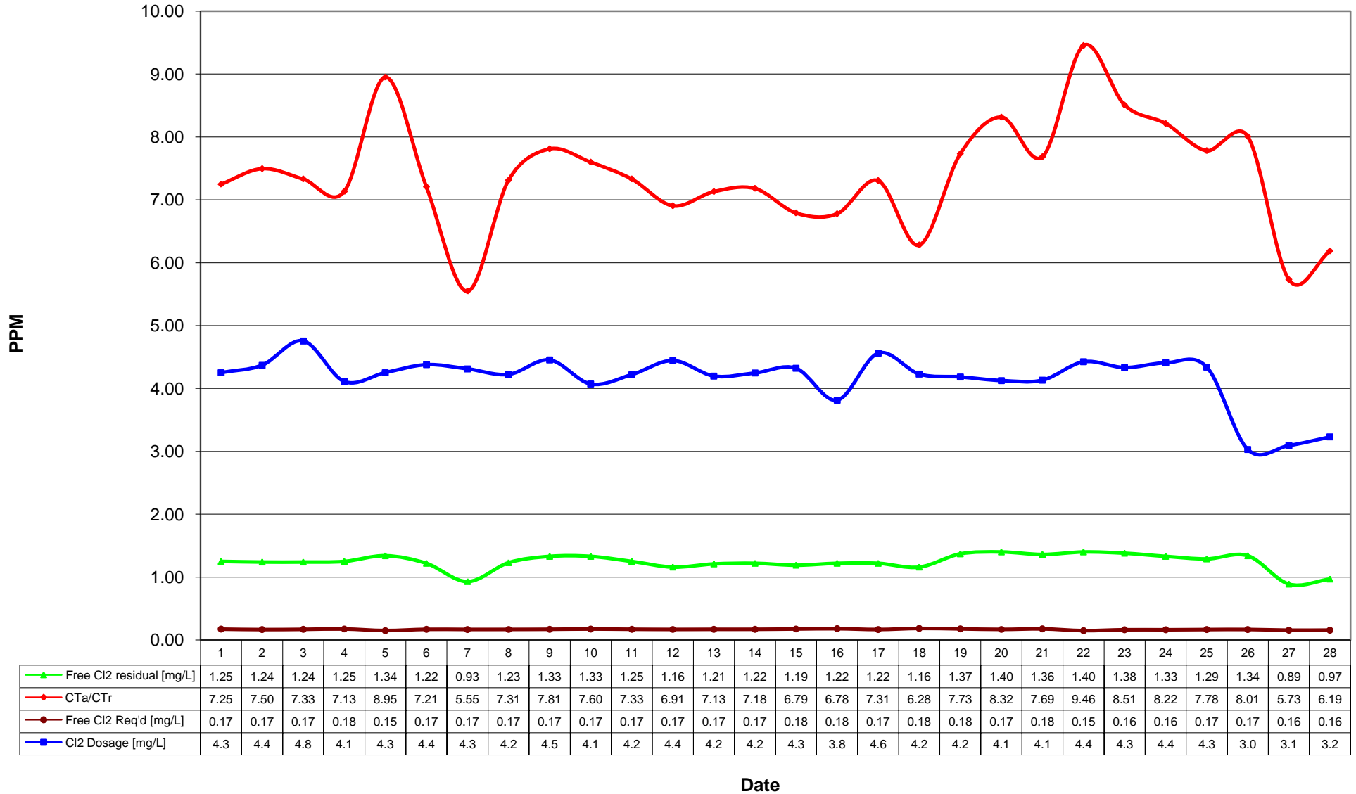
BMID CxT Chart February 2008 Mission Creek Source
