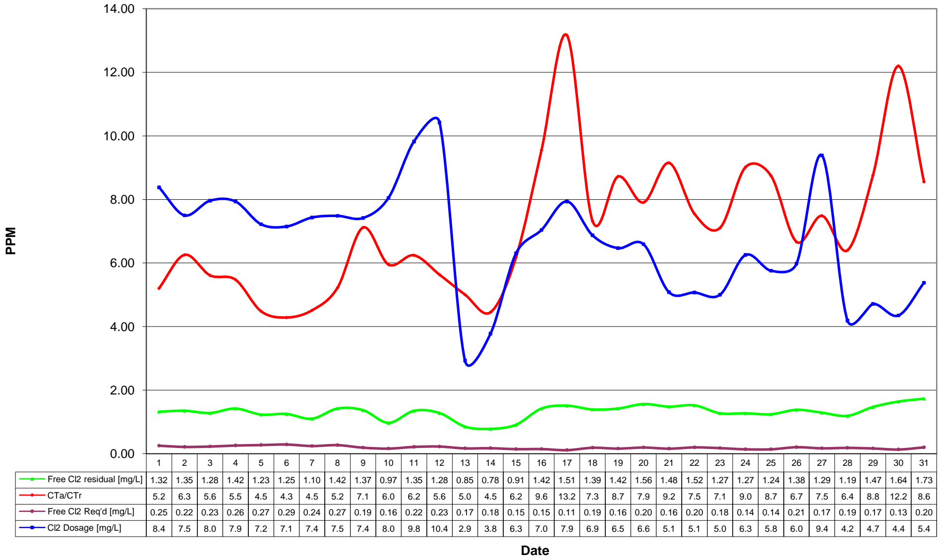
BMID CxT Chart October 2010 Mission Creek Source
