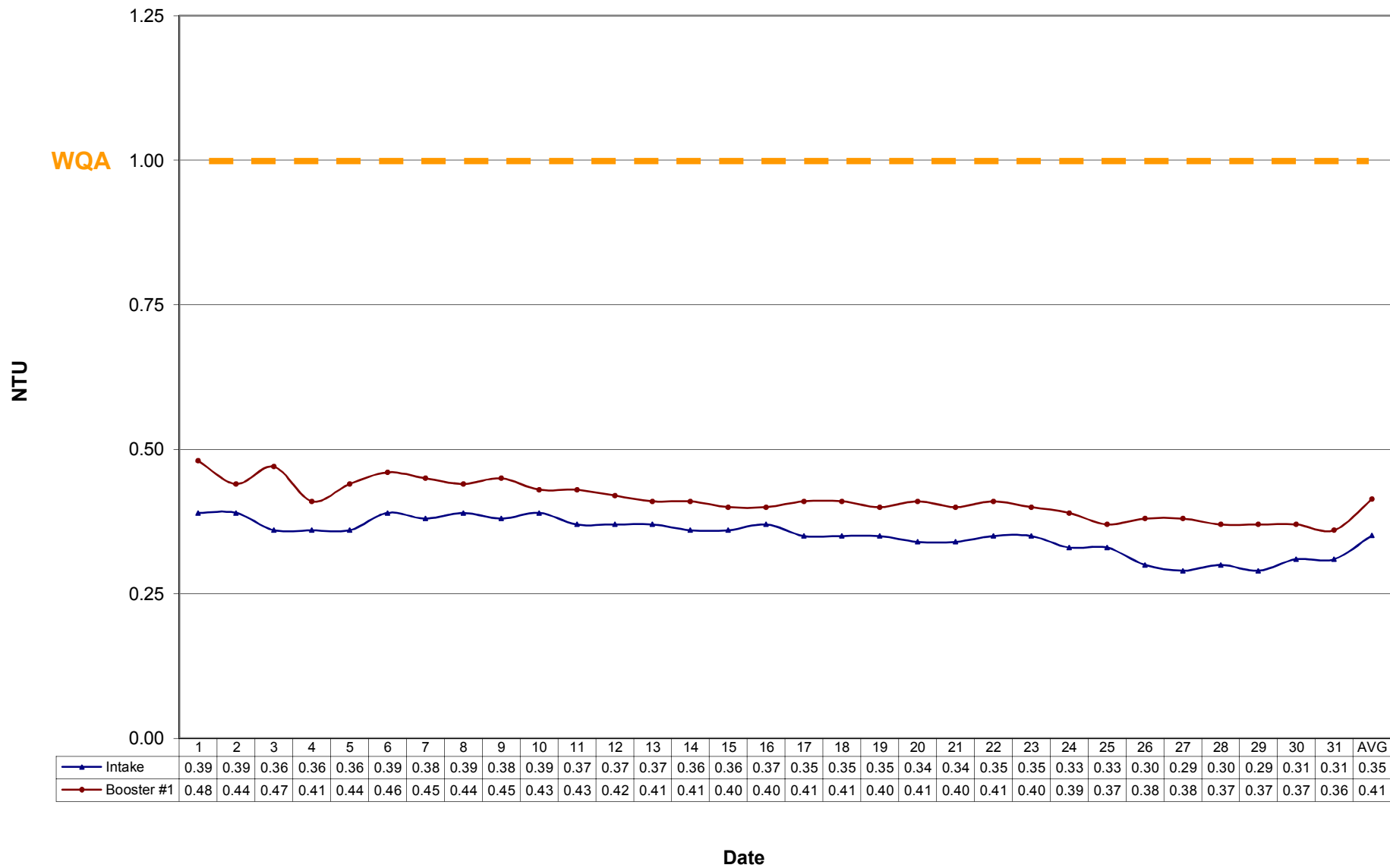
BMID Turbidity October 2011 (Single Point Daily Sampling with Inline Hach 1720c)
