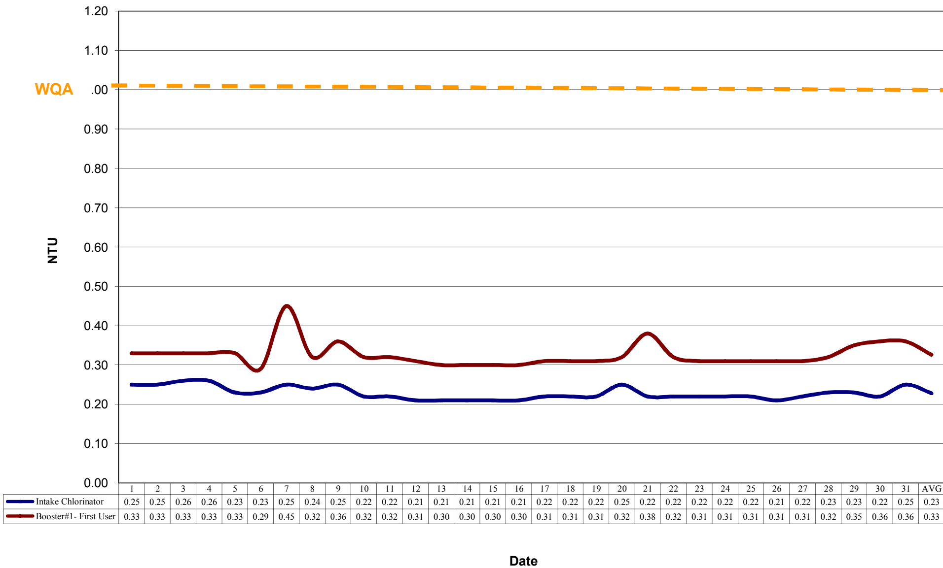
BMID Turbidity December 2011 (Single Point Daily Sampling with Inline Hach 1720c)
