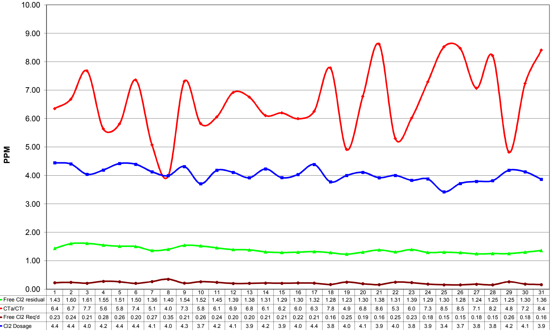
BMID CxT Chart January 2013 Mission Creek Source
