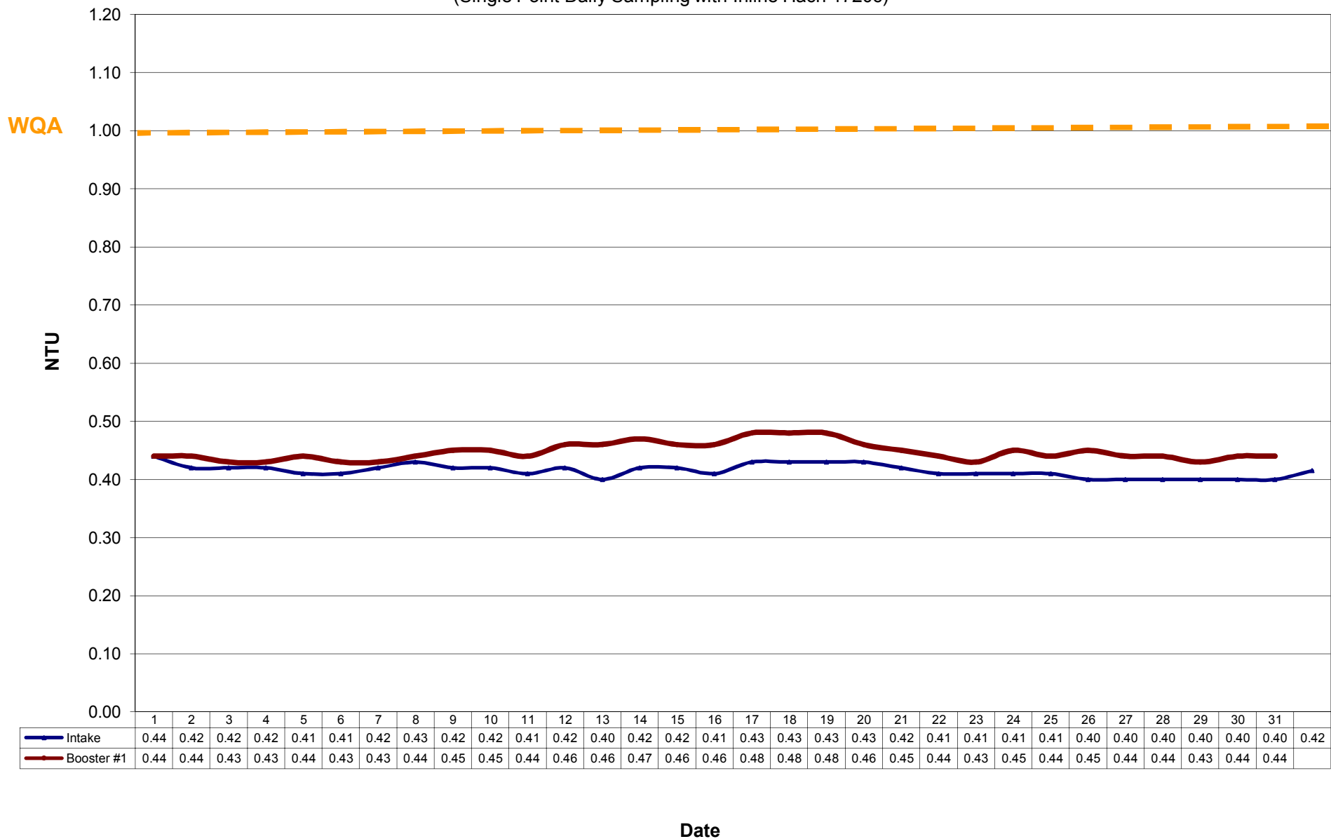
BMID Turbidity January 2014 (Single Point Daily Sampling with Inline Hach 1720c)
