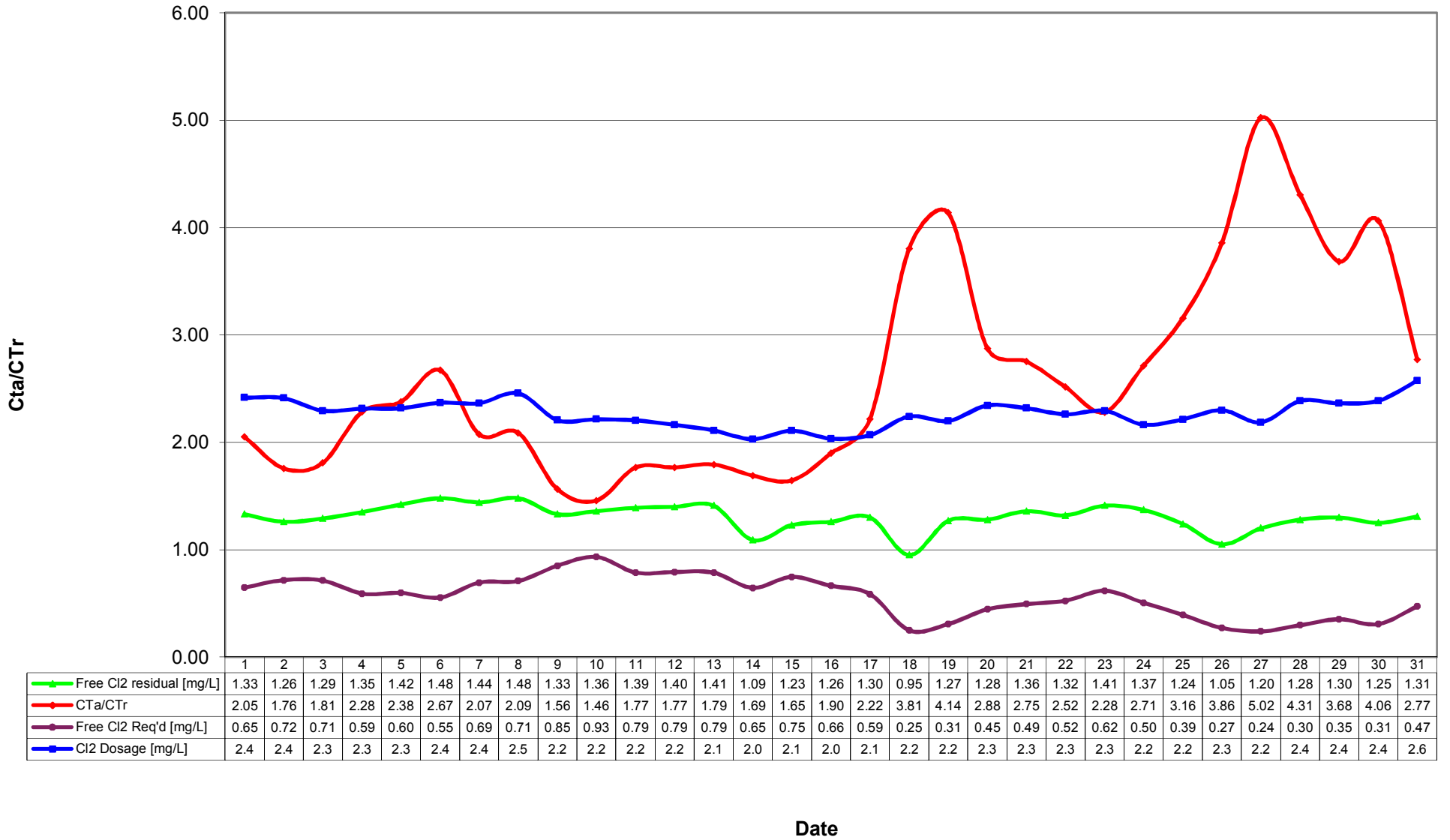
BMID CxT Chart May 2015 Mission Creek Source
