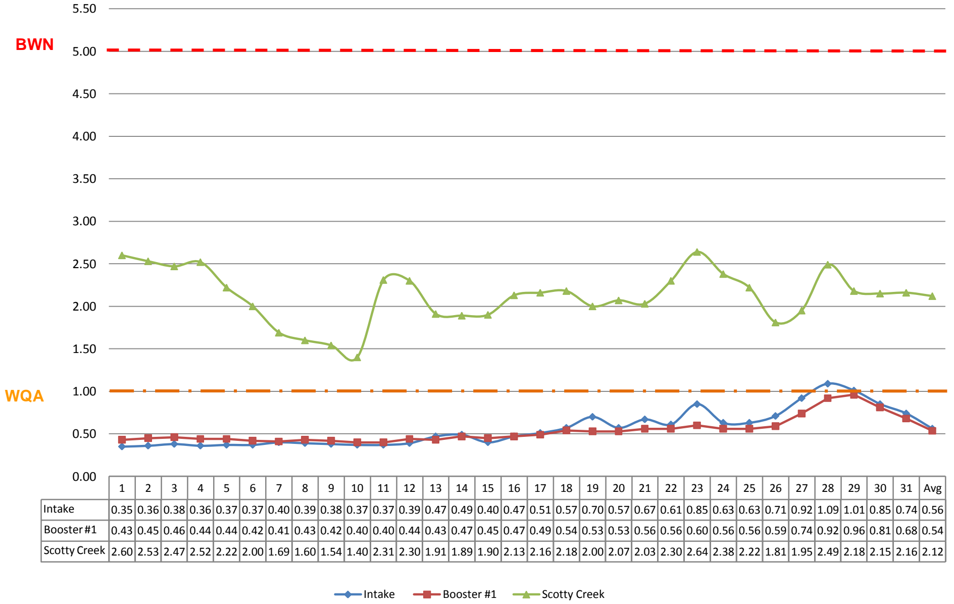
BMID Turbidity July 2009 (Single Point Daily Sampling with Inline Hach 1720c)
