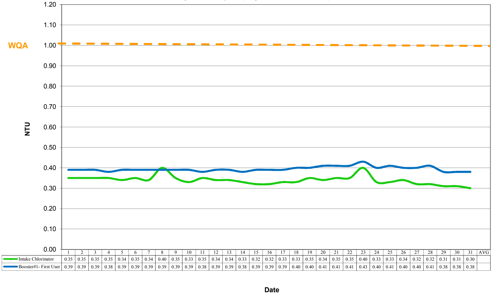
BMID Turbidity December 2015 (Single Point Daily Sampling with Inline Hach 1720c)
